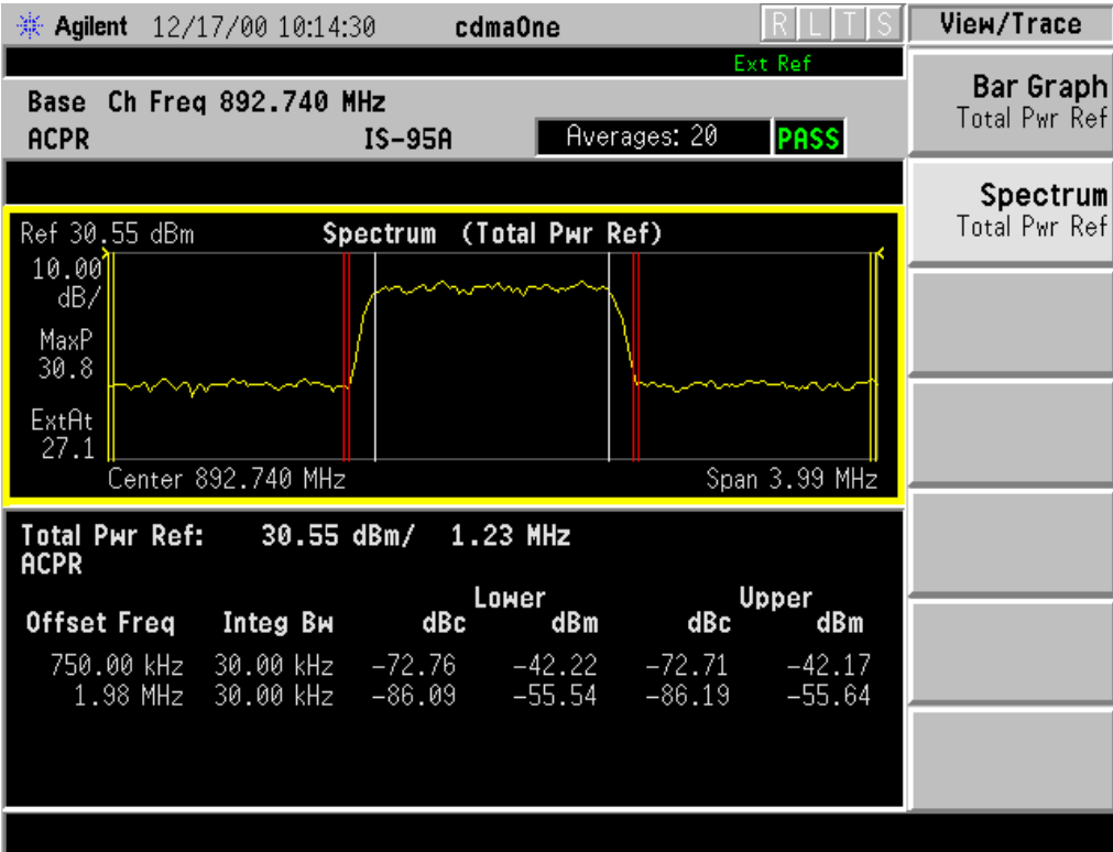
Figure 3-14 Adjacent Channel Power Ratio Measurement - Spectrum View
